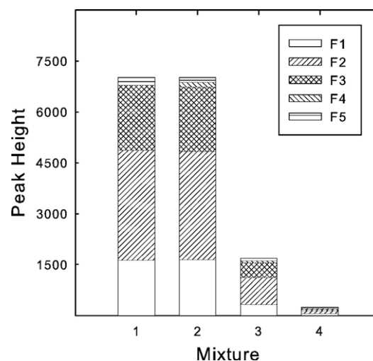
Fig. 2. Observed peak heights of five different fungal species (F1 — Fusarium equiseti , F2 — Alternaria solani , F3 — Verticillium sp., F4 — Rhizoctonia solani , F5 — Sclerotinia sclerotium ) from mixed-template PCR reactions. Mixture compositions are shown in Table 2.
