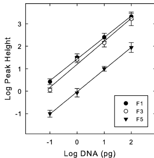
Fig. 3. Relationship between peak height and starting DNA template concentration for three pure fungal cultures. (F1 — Fusarium equiseti : y=1.430+0.960x , R^2=0.998 ; F3 — Verticillium sp.: y=1.195+1.025x , R^2=0.988 ; F5 — Sclerotinia sclerotium : y=-0.0270+0.989x , R^2=0.999 ).
