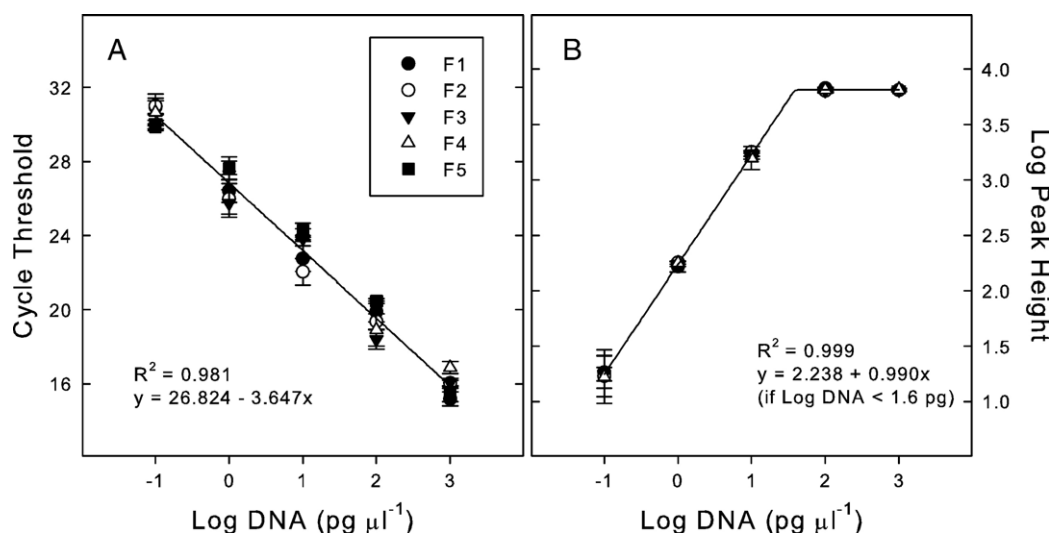
Fig. 1. Relationship between starting template concentration and cycle threshold (panel A) or peak height (panel B). DNA was isolated from pure cultures of five different species (F1 — Fusarium equiseti , F2 — Alternaria solani , F3 — Verticillium sp., F4 — Rhizoctonia solani , F5 — Sclerotinia sclerotium ).
